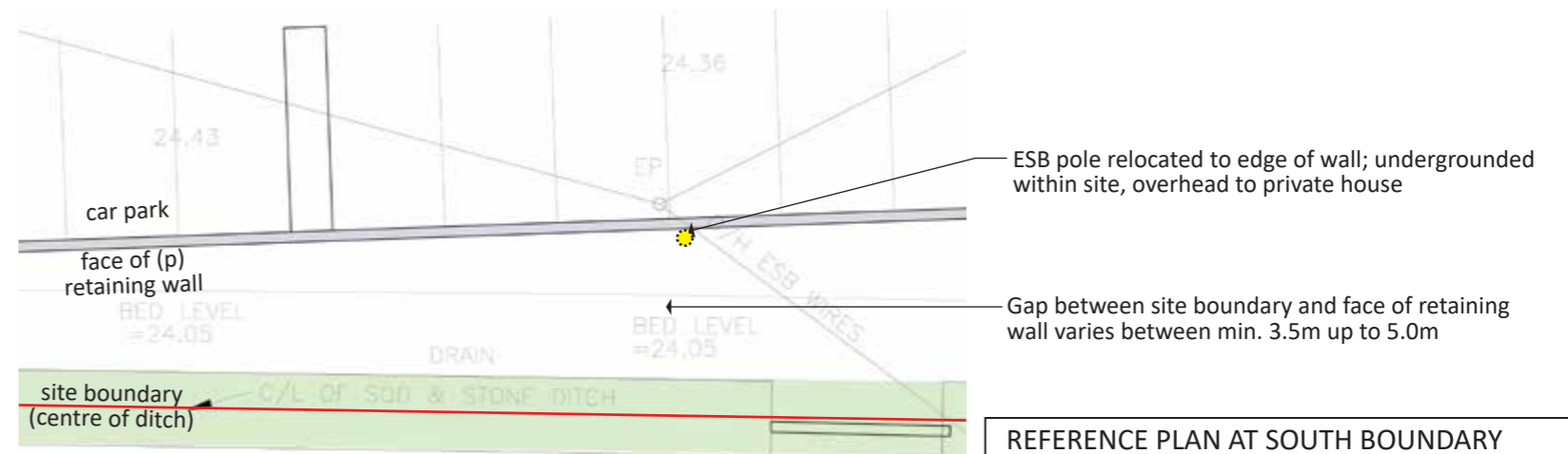
Extract of layout plan superimposed on site survey. This portion of boundary generally represents the extent of the image in the photo at left.
